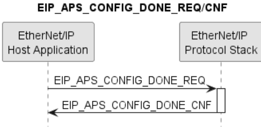
Figure 13. Sequence Diagram for the EIP_APS_CONFIG_DONE_REQ/CNF Packet
