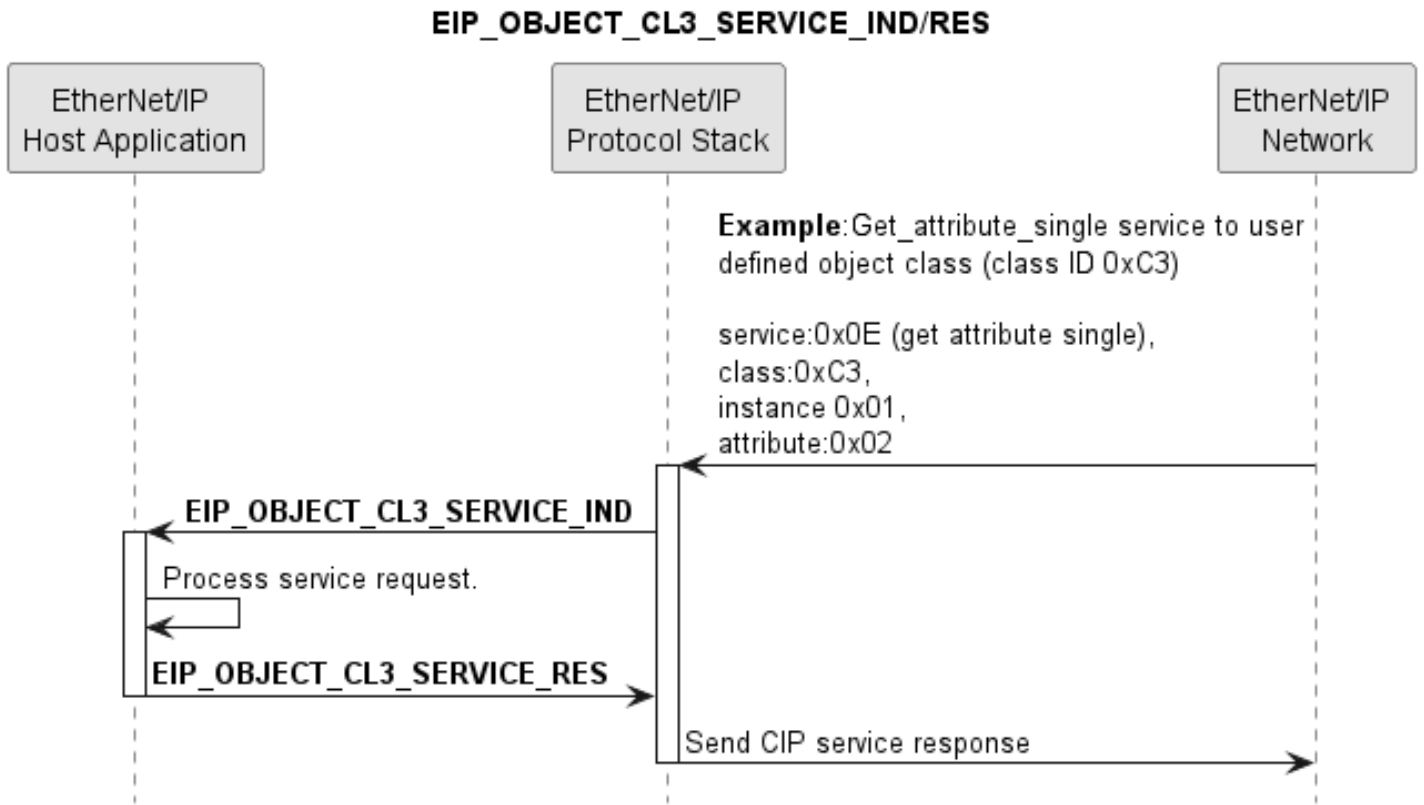
Figure 15. Sequence Diagram for the EIP_OBJECT_CL3_SERVICE_IND/RES Packet for the Extended Packet Set
