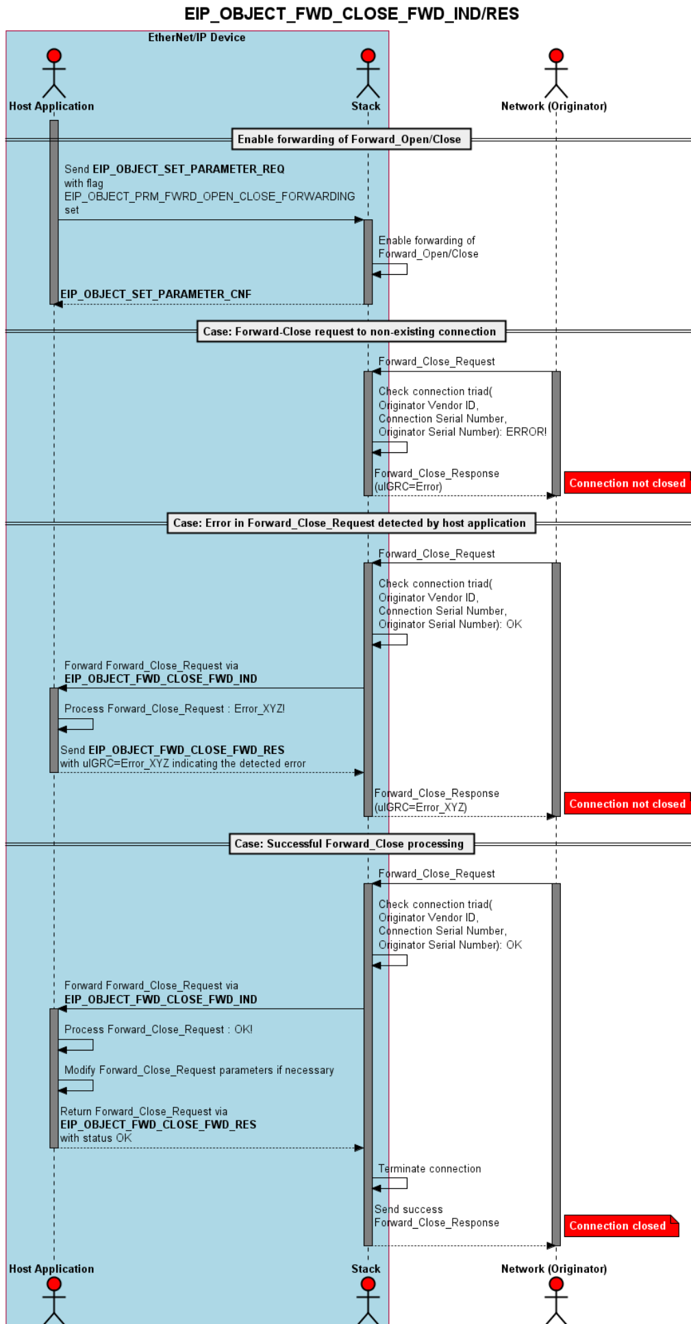
Figure 17. Packet sequence for Forward_Close forwarding functionality
