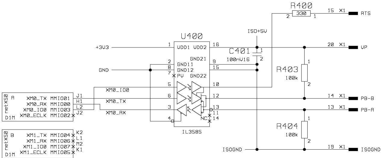
Figure 49: Plan of PROFIBUS DP Interface of NIC 50-DPS
