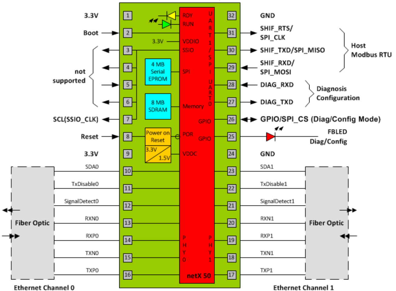
Figure 27: NIC 50-REFO Block Diagram - External Connections and internal Structure
