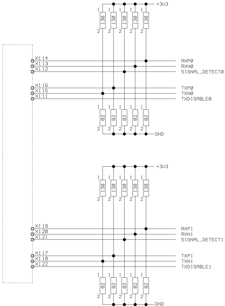
Figure 29: Proposal for the Design connecting the optical Real-Time-Ethernet Interface of the NIC 50-REFO with a fiber-optical Transceiver
