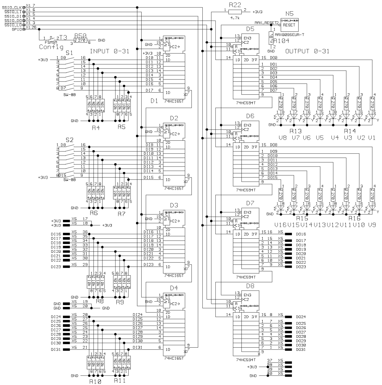
Figure 65: Wiring Diagram of the Serial I/O Shift Register-Interface of the Evaluation Board
