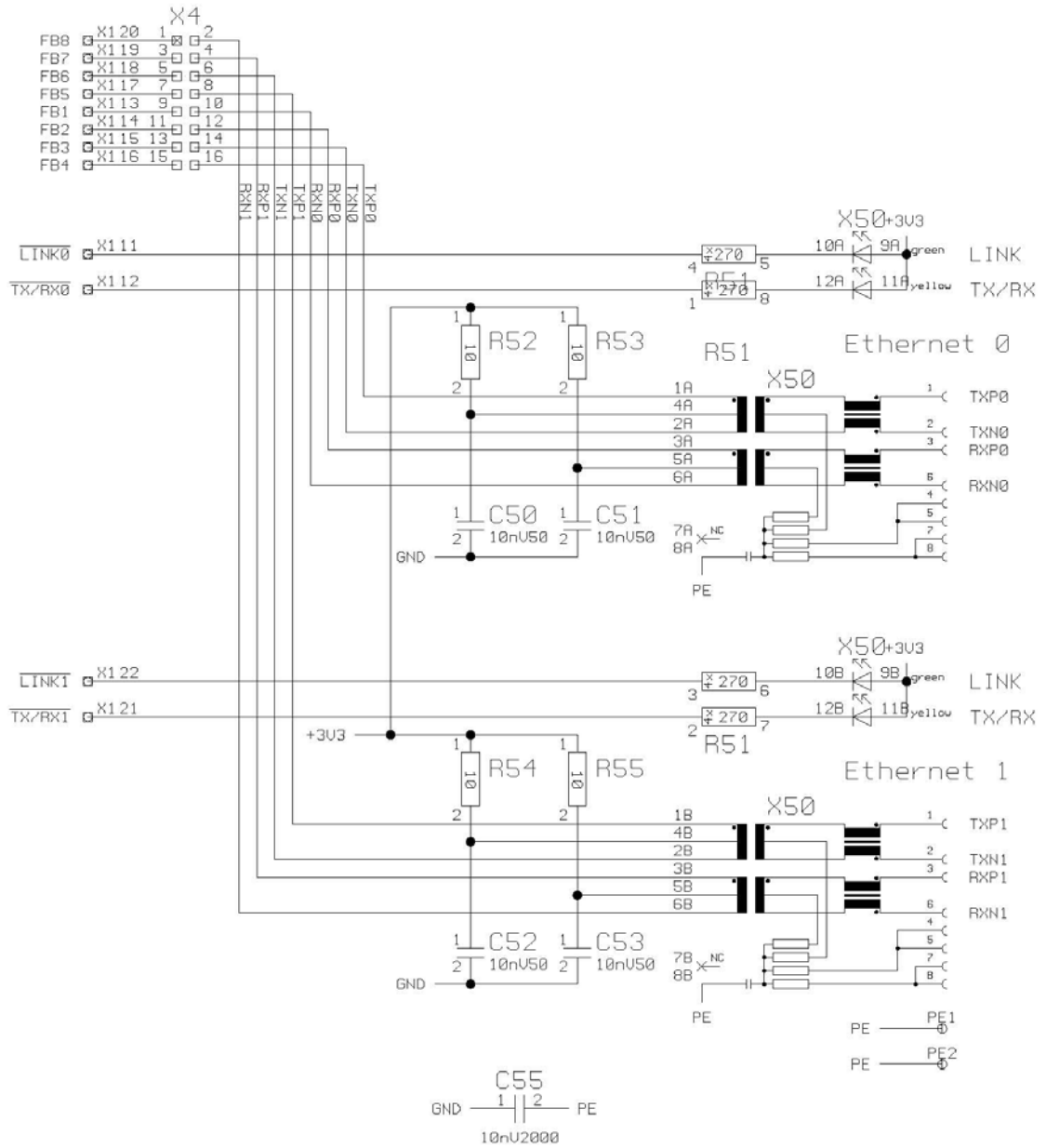
Figure 67: Wiring Diagram of the Ethernet-Interface of the Evaluation Board NICEB
