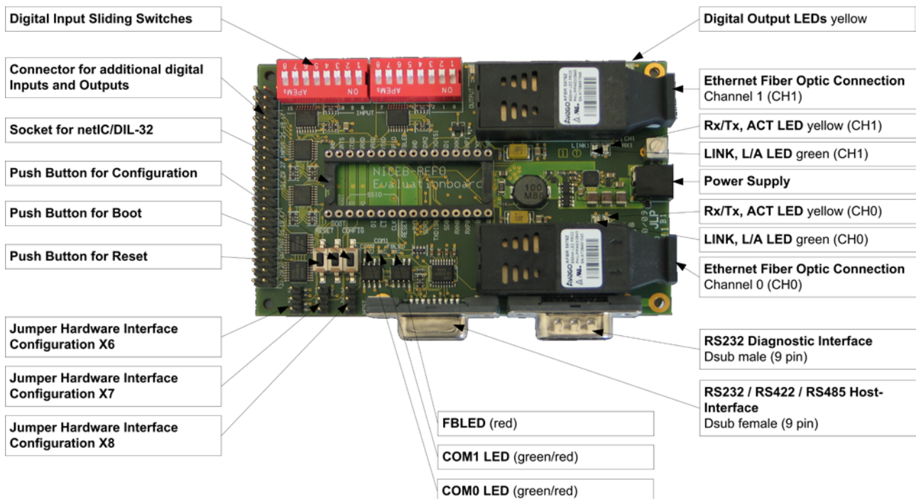
Figure 68: Device Photo Evaluation Board NICEB-REFO
