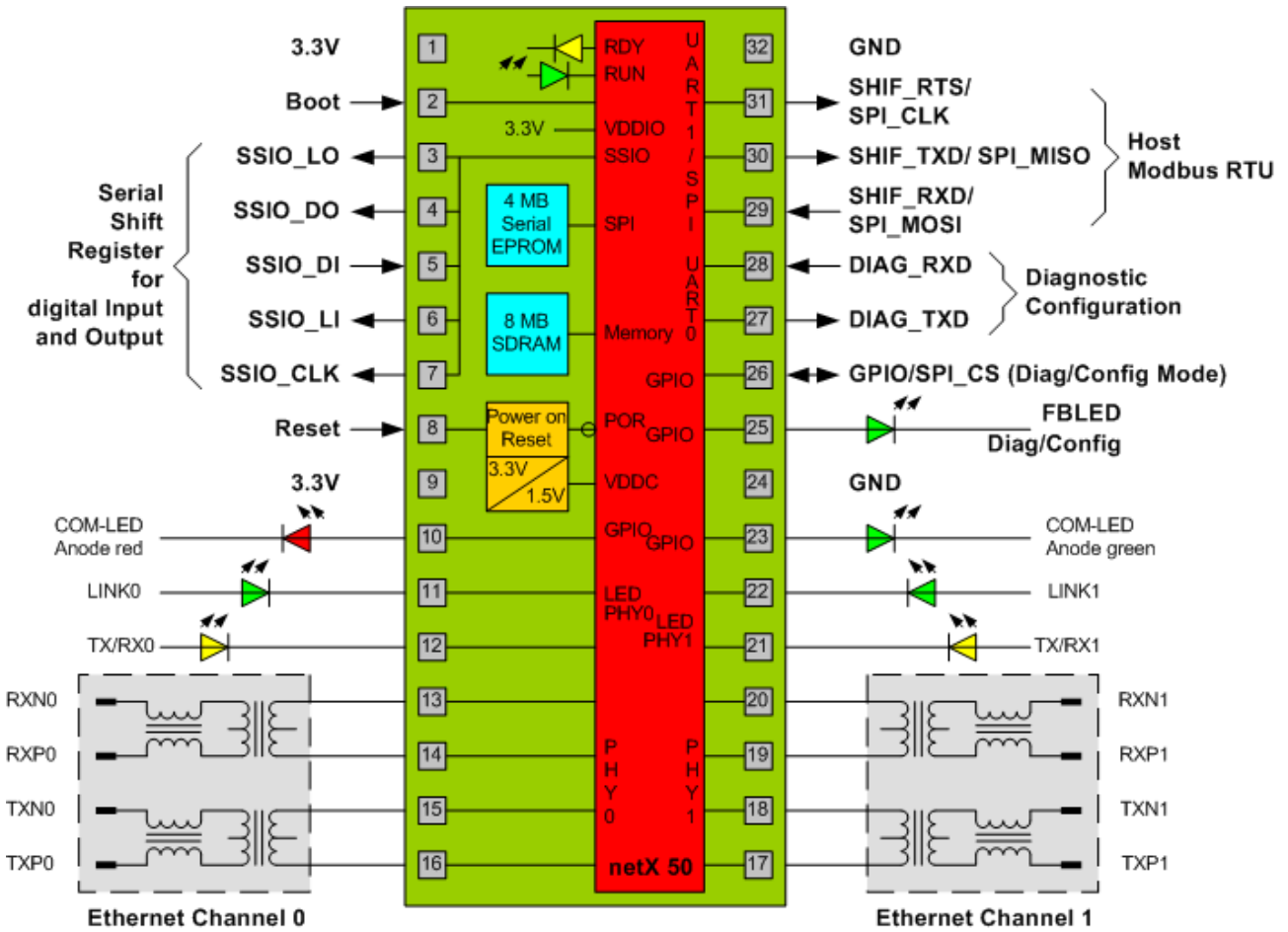
Figure 53: NIC 52-RE Block Diagram - External Connections and internal Structure
