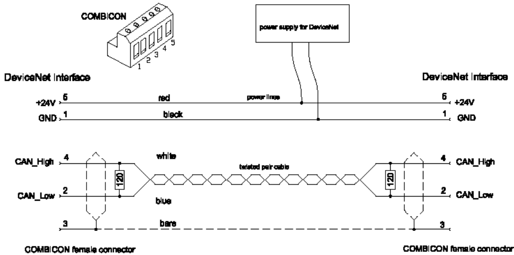
Figure 78: DeviceNet Network
