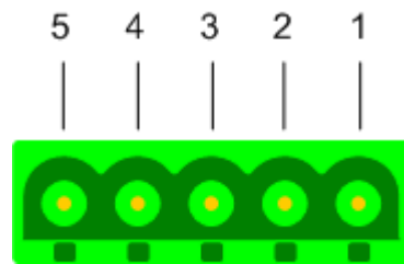
Figure 77: DeviceNet Interface (CombiCon male Connector, 5 pin) of NICEB-AIF-DN
