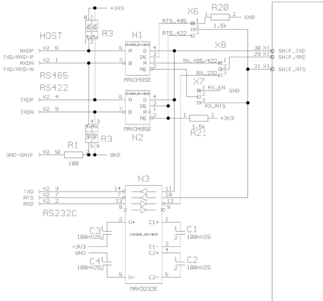
Figure 64: Wiring Diagram of the Serial Host-Interface of the Evaluation Board
