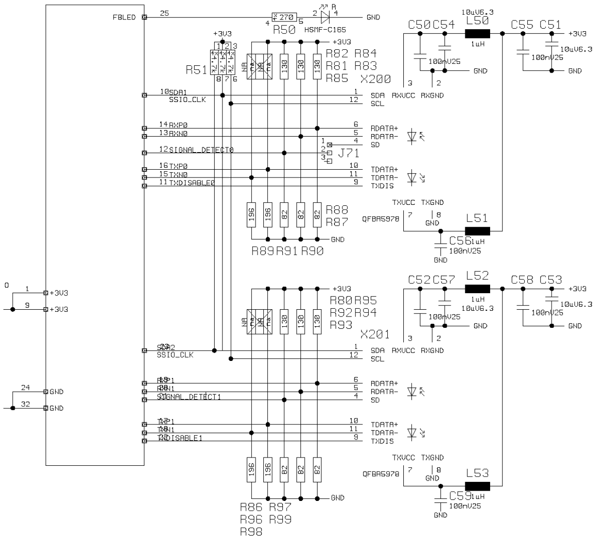
Figure 69: Coupling the netIC to optical Transceivers
