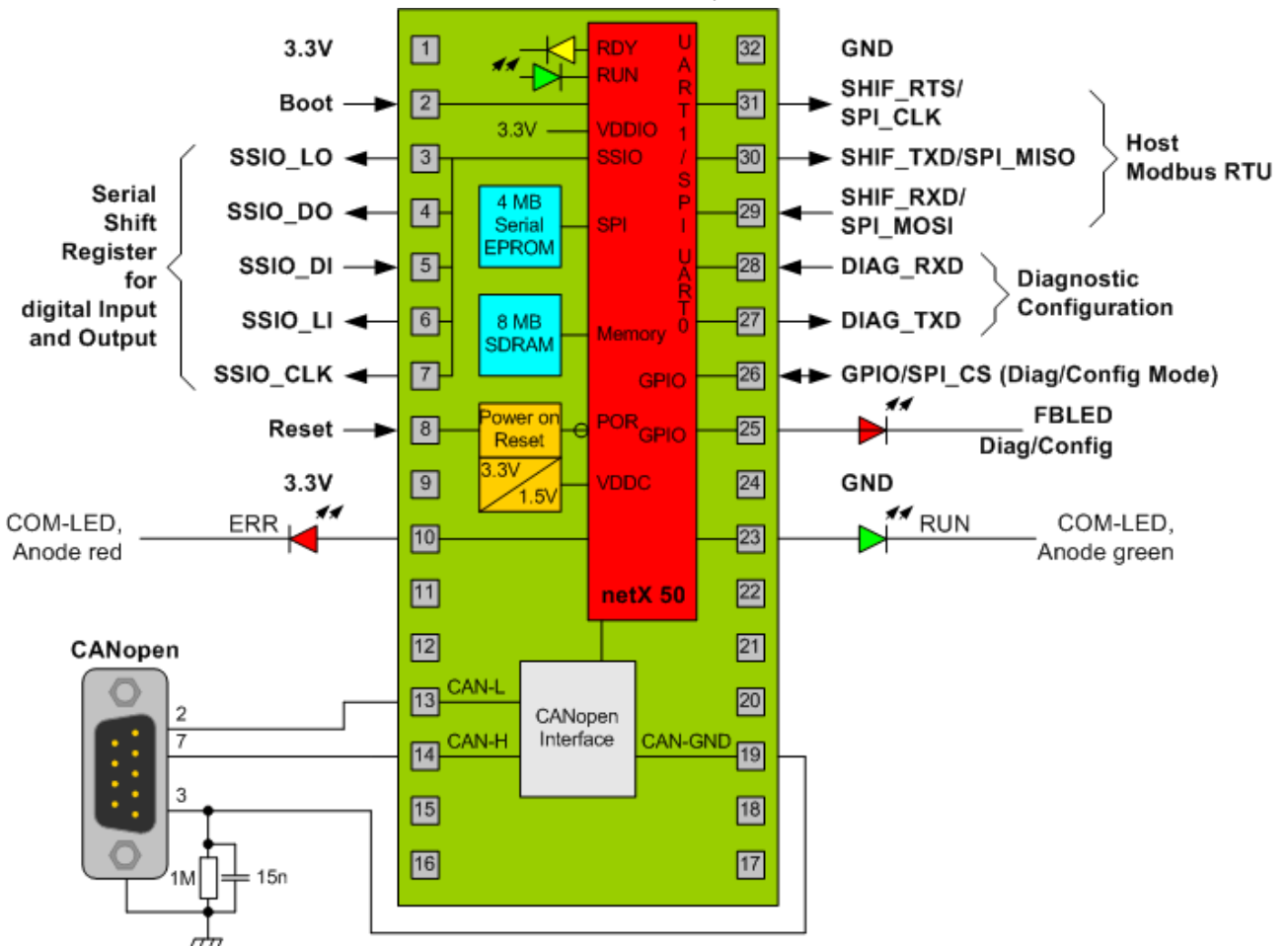
Figure 37: NIC 50-COS Block Diagram - External Connections and internal Structure
