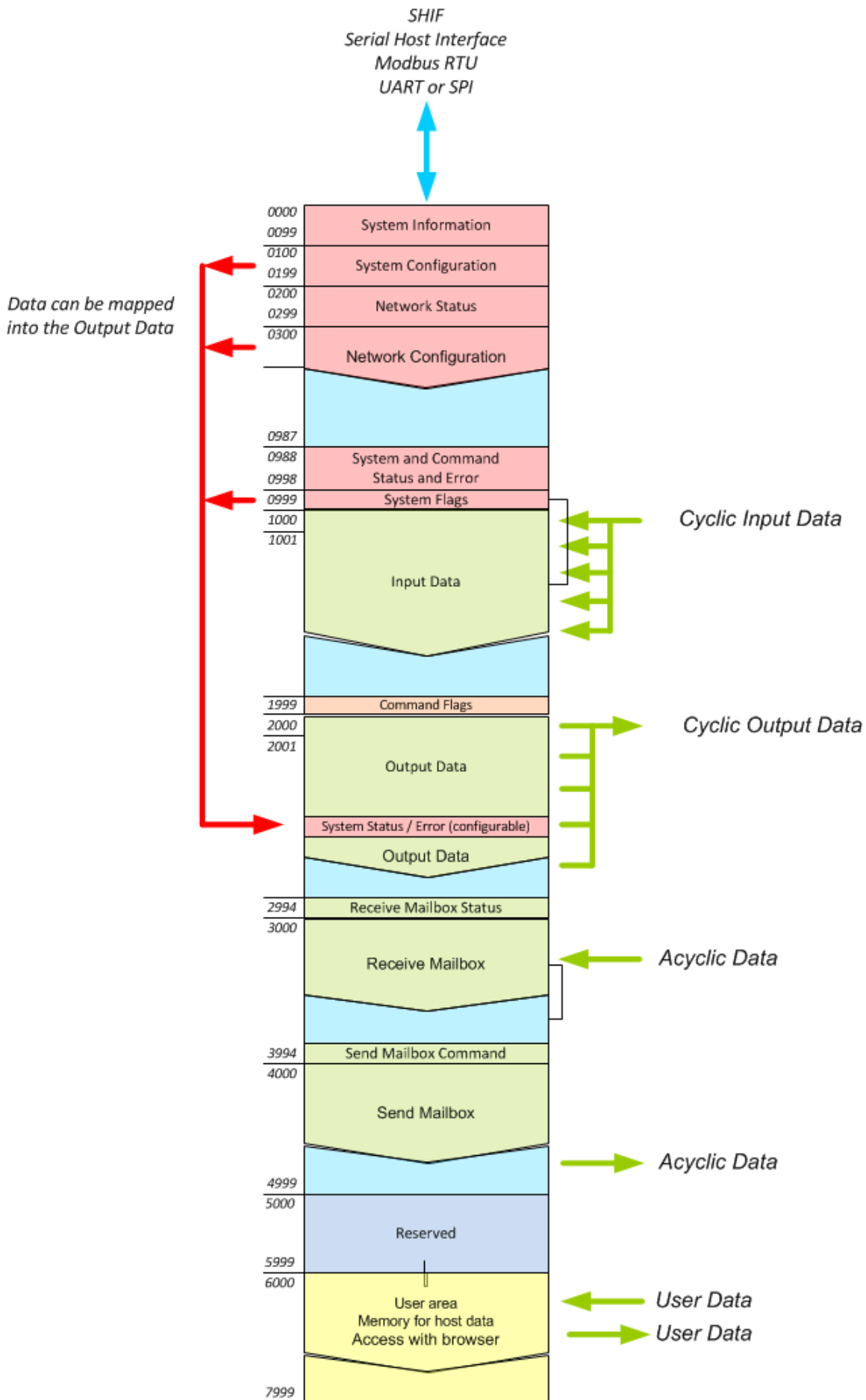
Figure 6: Register Area
