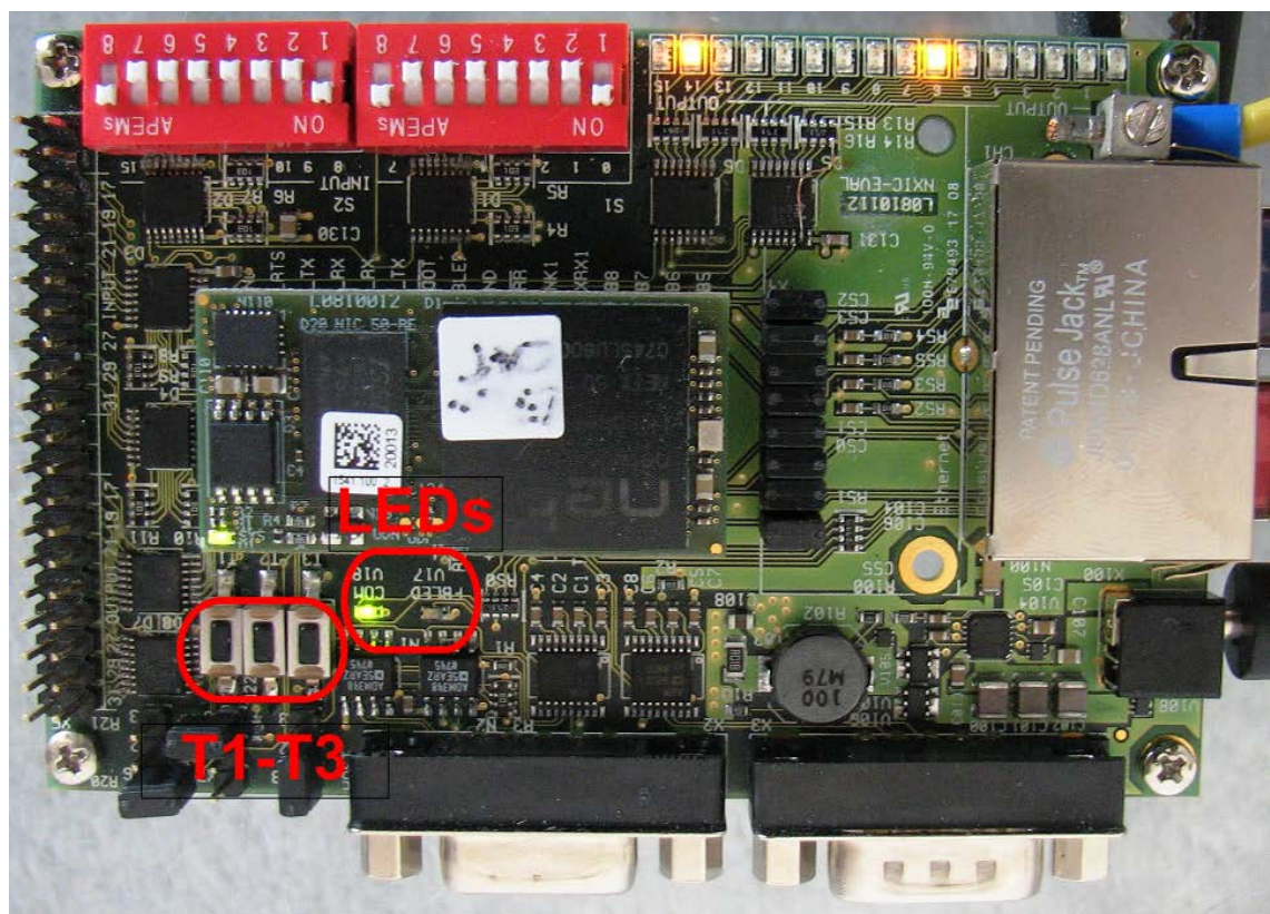
Figure 60: Photo of Evaluation-Board NICEB with Positions of Switches T1-T3 and LEDs
