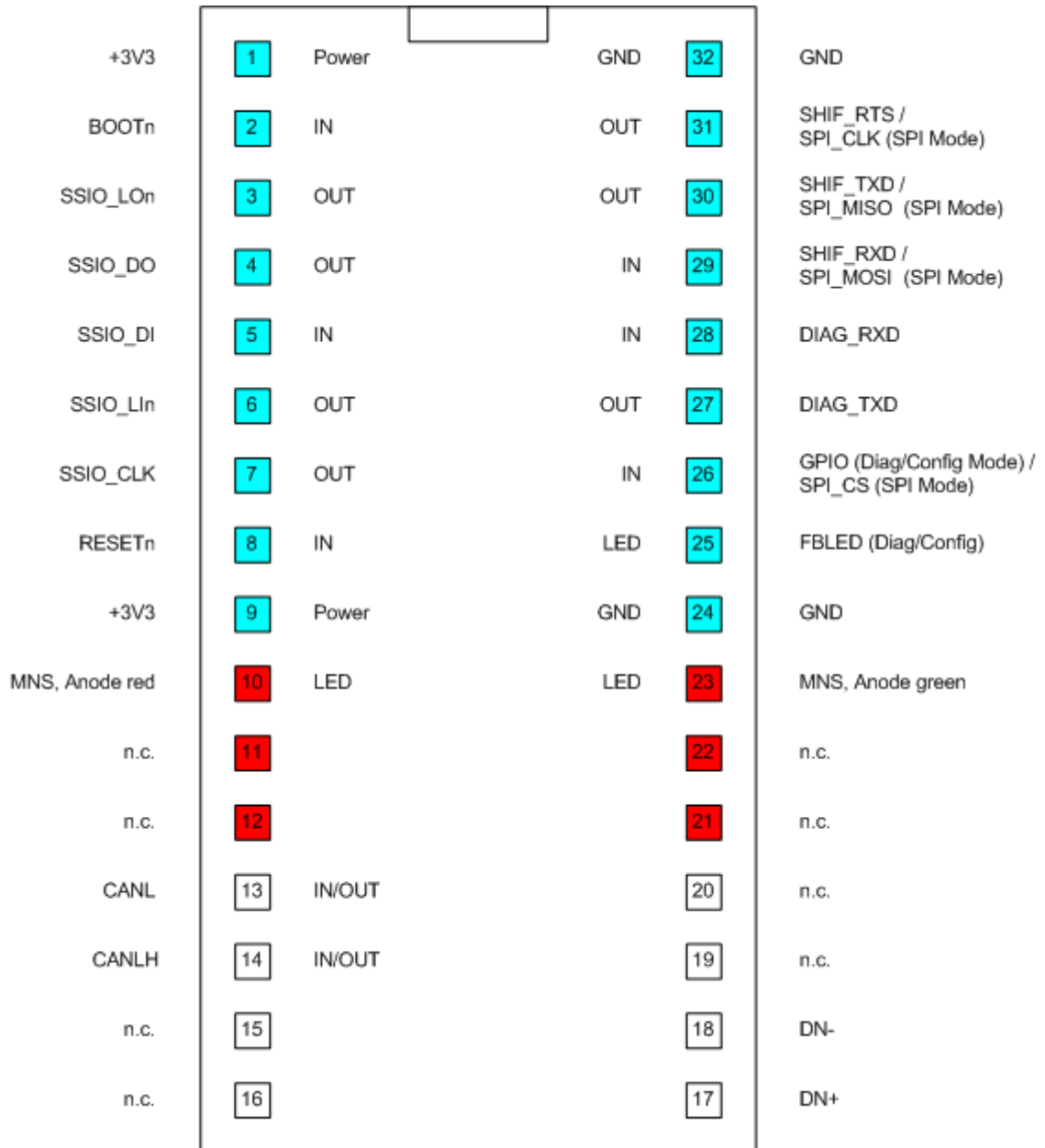
Figure 43: Pinning of NIC 50-DNS
