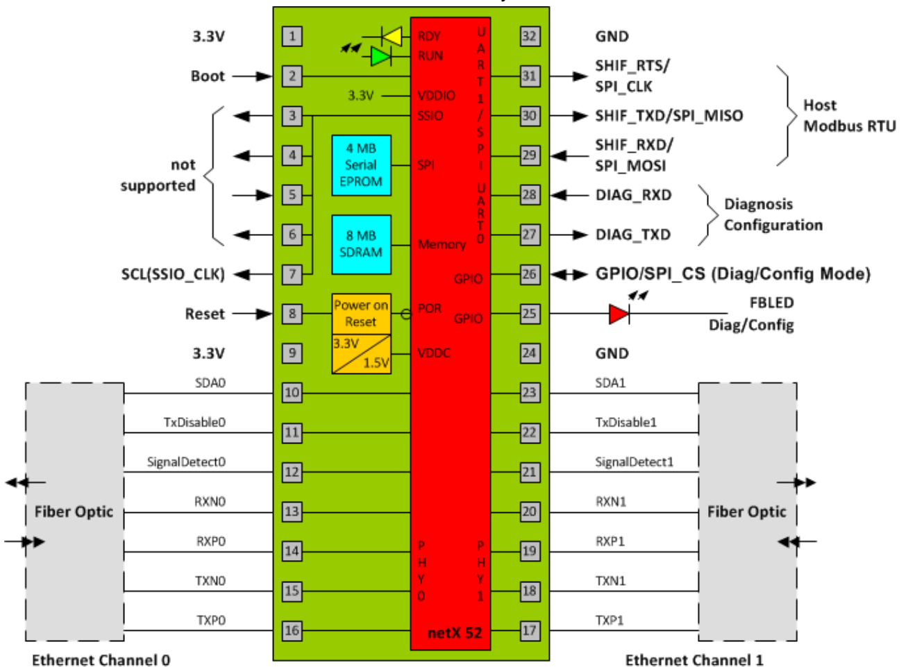
Figure 56: NIC 52-REFO Block Diagram - External Connections and internal Structure
