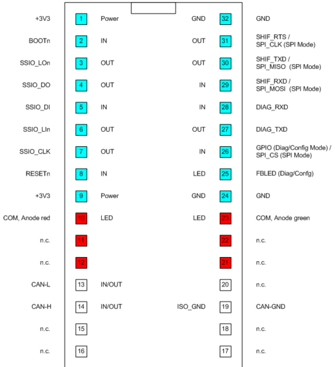
Figure 38: Pinning of NIC 50-COS
