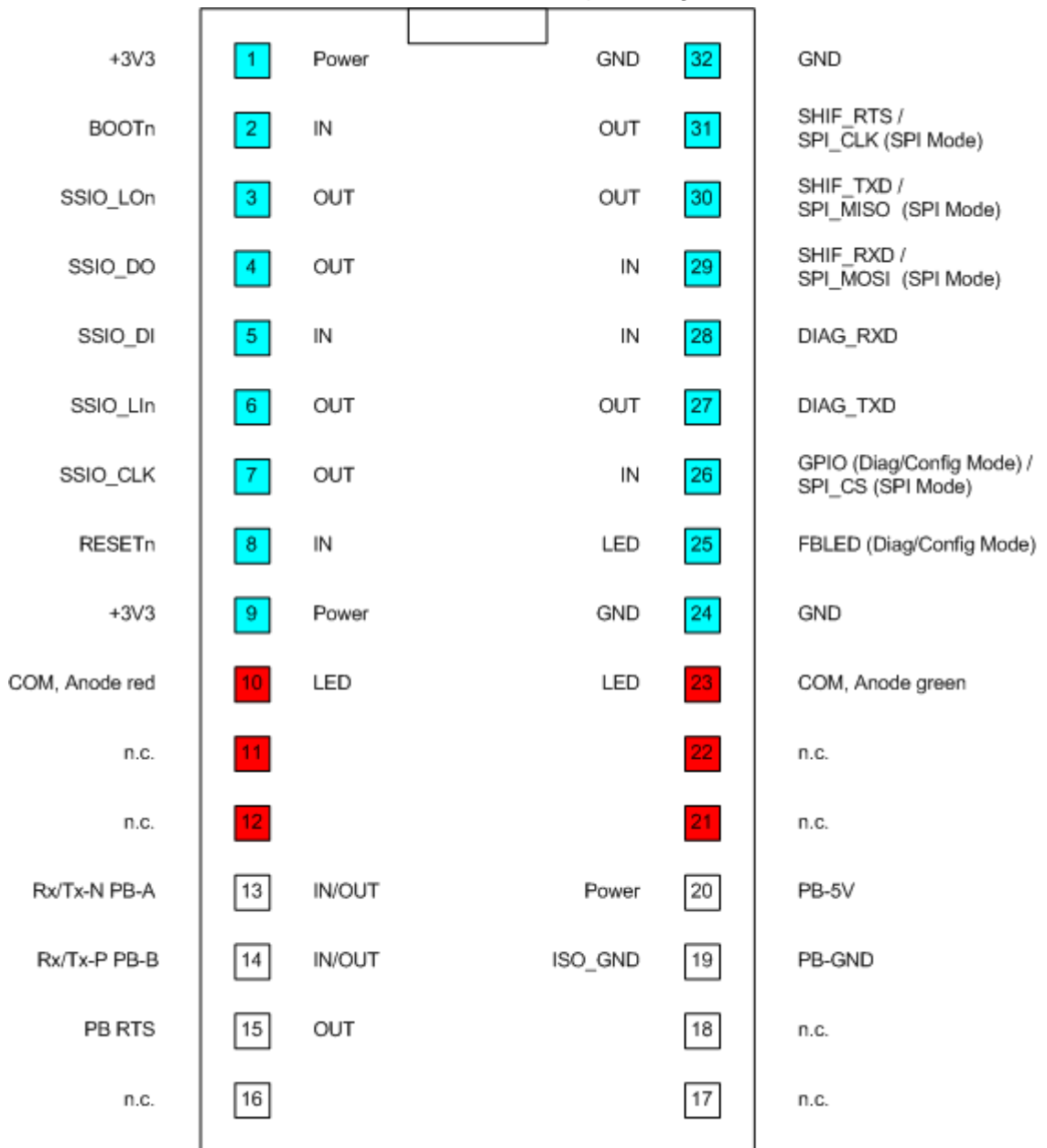
Figure 48: Pinning NIC 50-DPS
