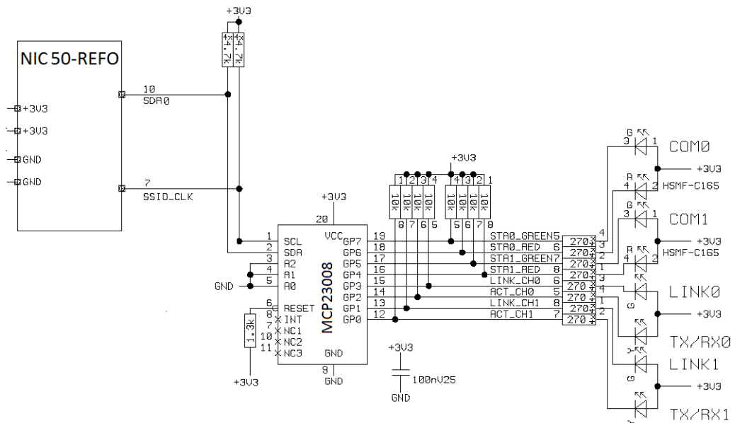
Figure 30: Connecting a LED Control for the NIC 50-REFO via I2C.
