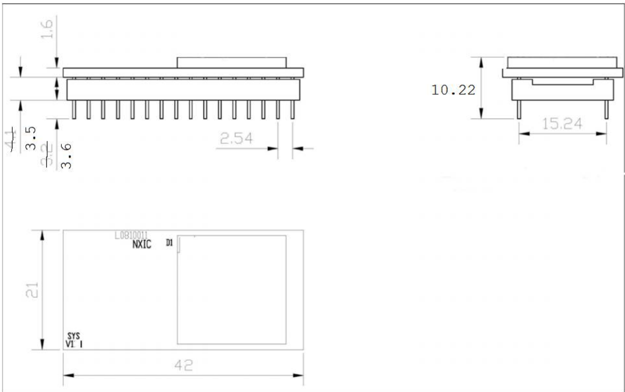
Abbildung 1: Dimensioned Device Drawing NIC 52-RE (top side)
