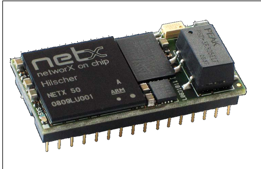
Figure 41: Photo NIC 50-DNS
