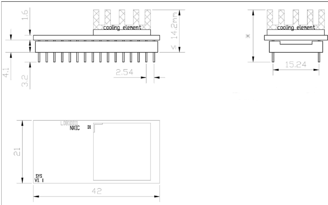
Figure 88: Device Drawing NIC 50-RE
