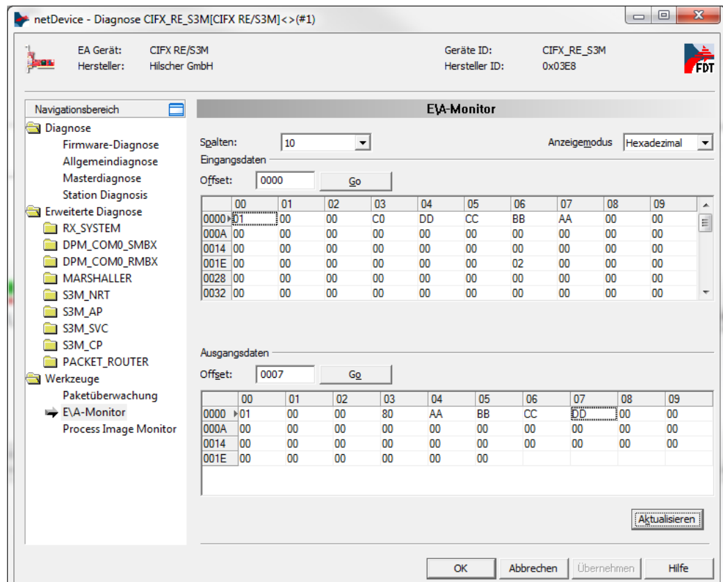
Figure 85: View of the Data of the Configuration Example in the IO Monitor of SYCON.net.
