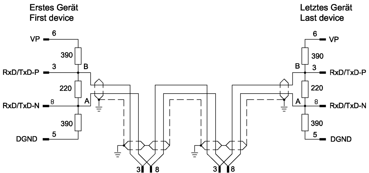
Figure 81: PROFIBUS-DP-Network
