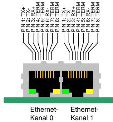
Figure 66: Schematic of Ethernet Connectors
