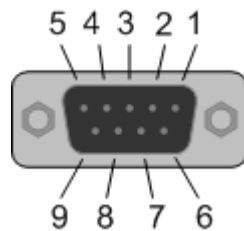
Figure 80: PROFIBUS-DP-Interface (D-Sub-female connector, 9-pole) of the NICEB-AIF-DP
