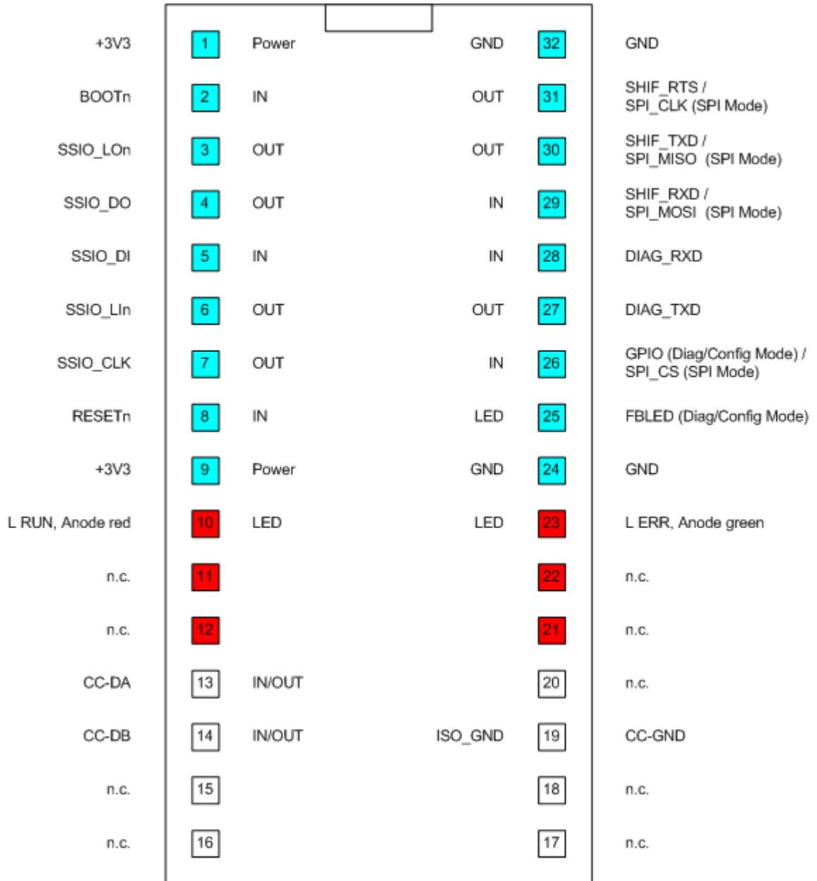
Figure 33: Pinning of NIC 10-CCS
