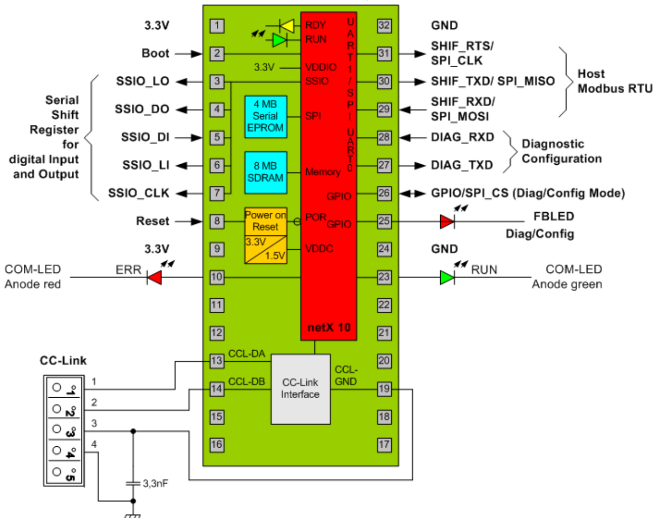
Figure 32: NIC 10-CCS Block Diagram - External Connections and internal Structure
