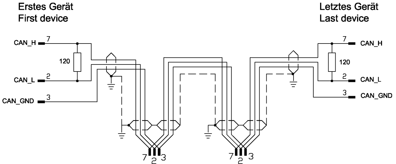
Figure 75: CAN- Network
