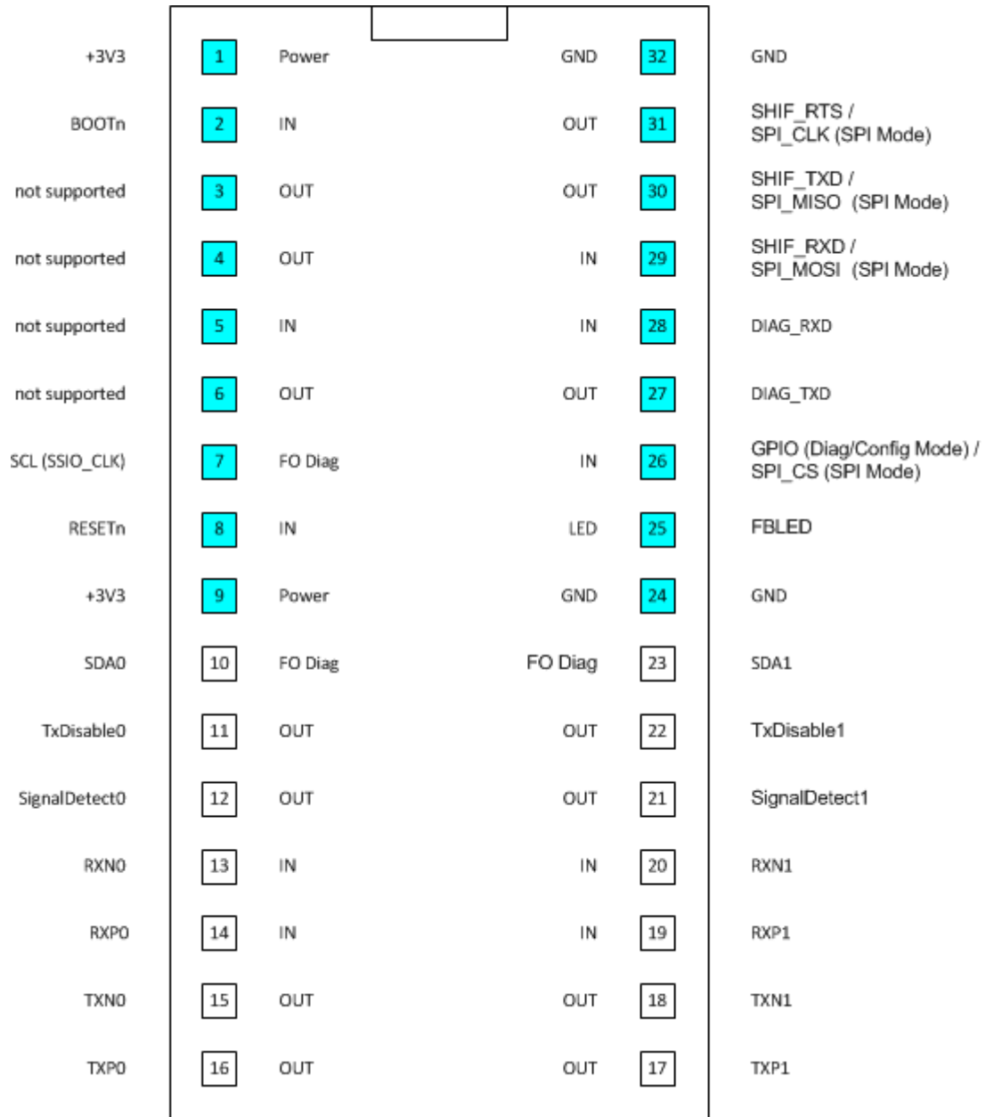
Figure 28: Pinning of NIC 50-REFO
