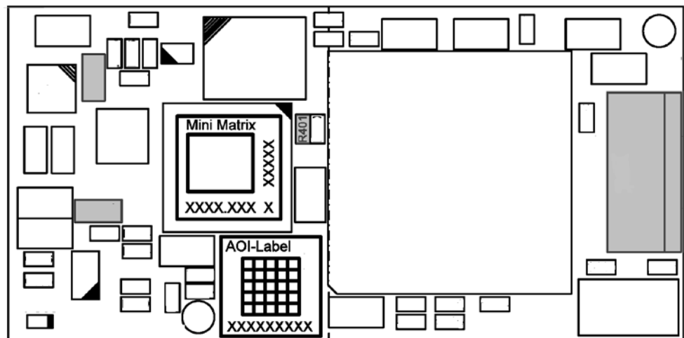
Figure 96: Dimensioned Device Drawing NIC 52-RE (top side)
