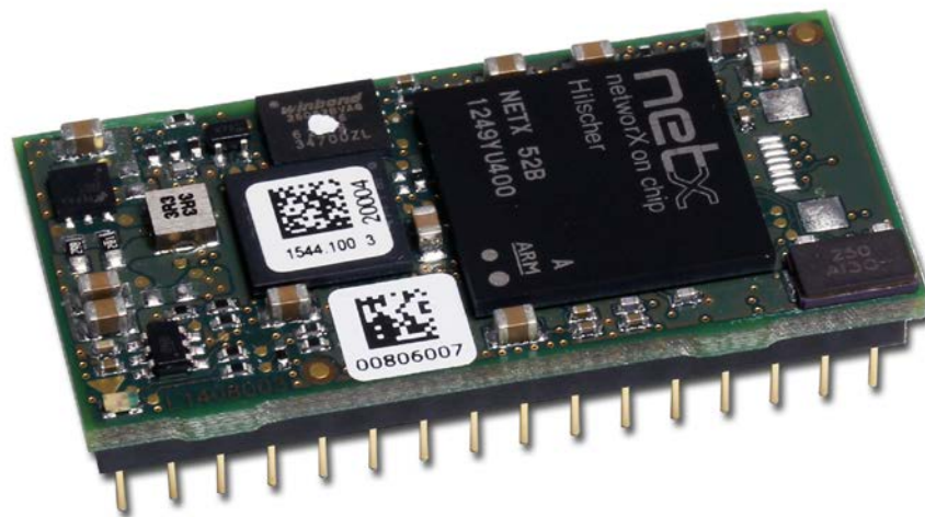
Figure 51: Photo NIC 52-RE (Top view)
