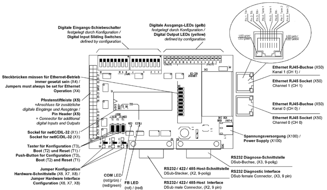
Figure 58: Device Drawing NICEB
