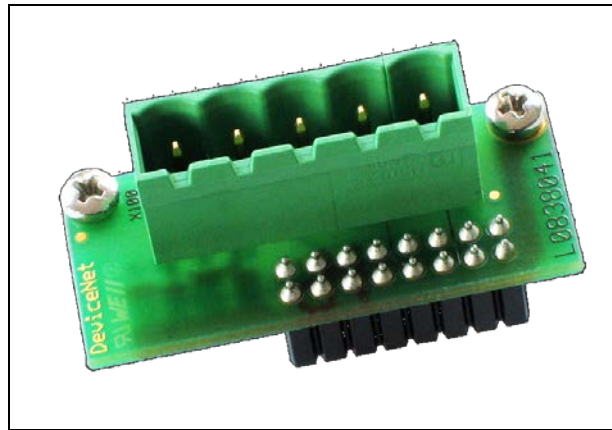
Figure 76: Photo DeviceNet-Adapter NICEB-AIF-DN
