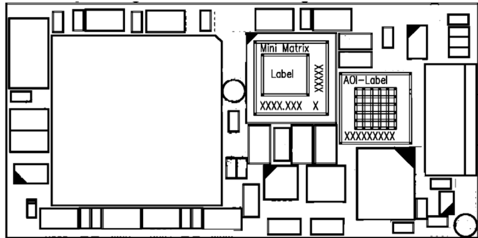
Figure 97: Device Drawing NIC 52-REFO (top side)
