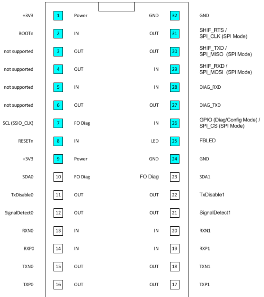
Figure 57: Pinning of NIC 52-REFO
