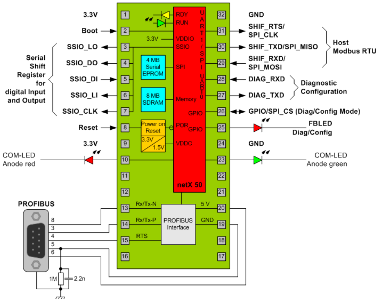
Figure 47: NIC 50-DPS Block Diagram - External Connections and internal Structure
