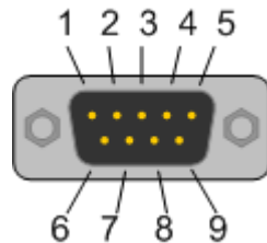
Figure 74: CANopen Interface (DSub male connector, 9 pin) of NICEB-AIF-CO
