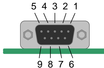
Figure 63: 9 Pin D-Sub Connector used as Host Interface Connector
