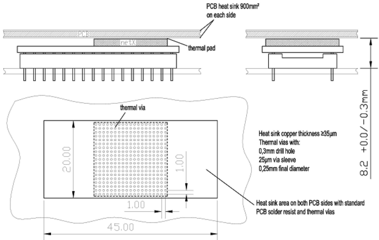
Figure 90: Device Drawing NIC 50-RE without Hilscher's original heat sink and over a PCB heat sink
