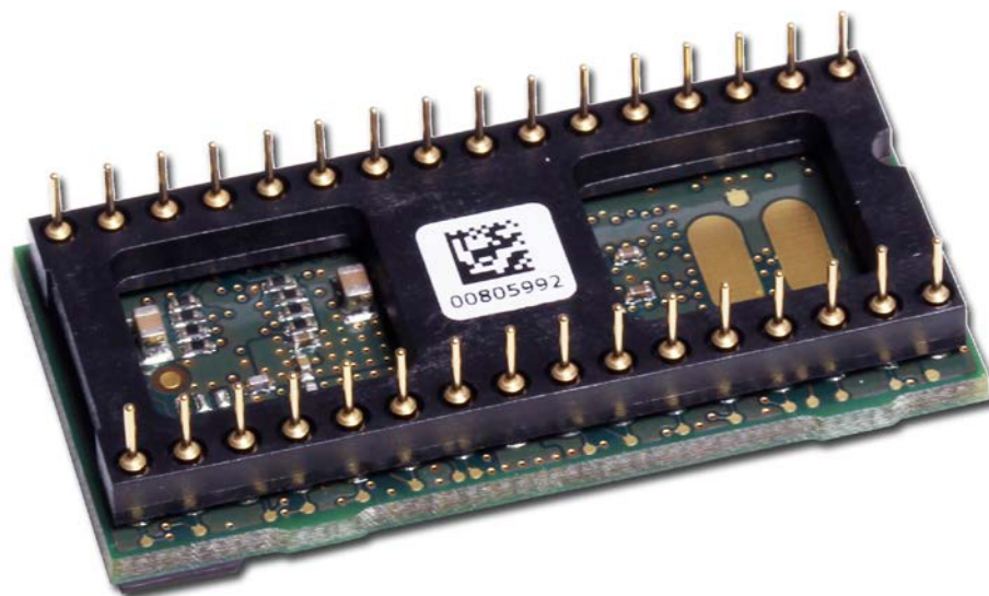
Figure 52: Photo NIC 52-RE (Bottom view)
