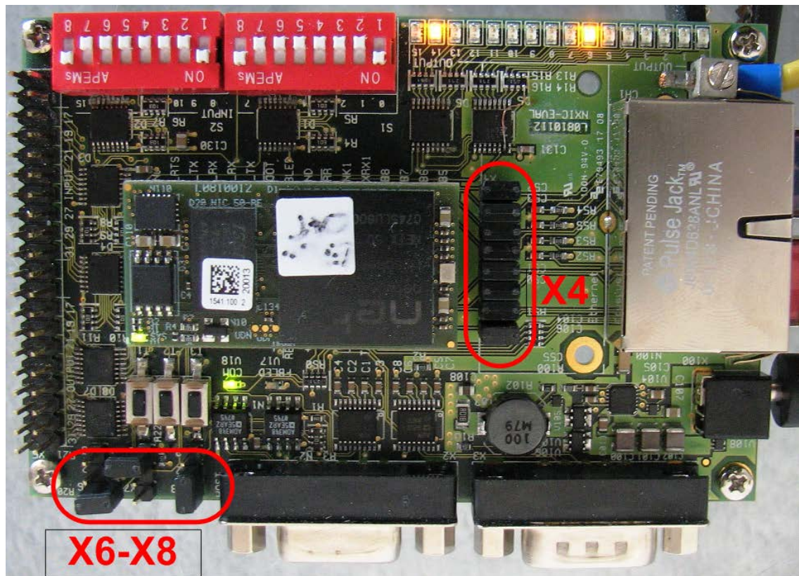
Figure 59: Photo of Evaluation-Board NICEB with Positions of Jumpers X4,X6-X8
