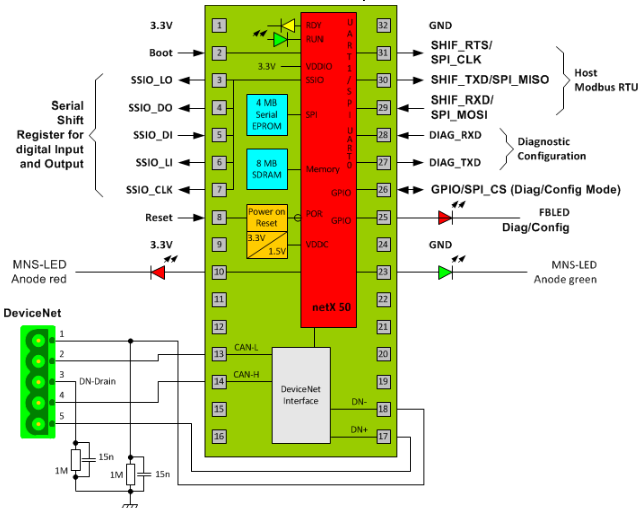
Figure 42: NIC 50-DNS Block Diagram - External Connections and internal Structure
